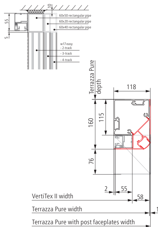
Top view of the VertiTex II rail guide on the example at Terrazza Pure front only
