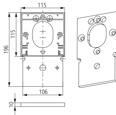
Post plate for 115 middle/wall post
