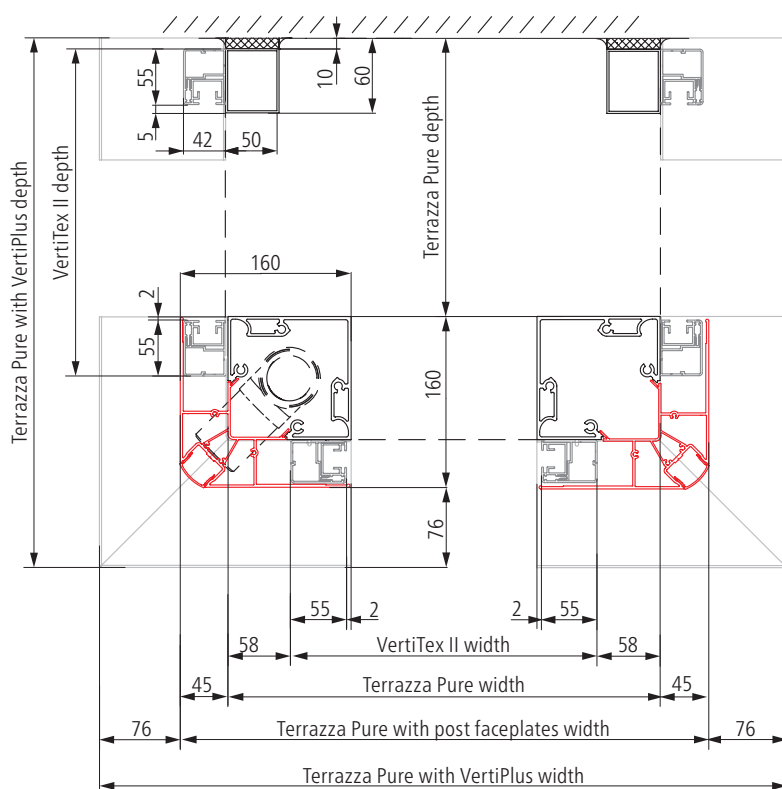
Top view of VertiTex II rail guide on the example at Terrazza Pure front and on the side
