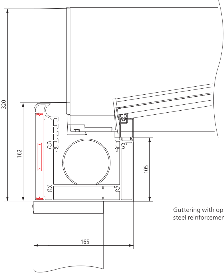
Guttering and wall bracket profiles
