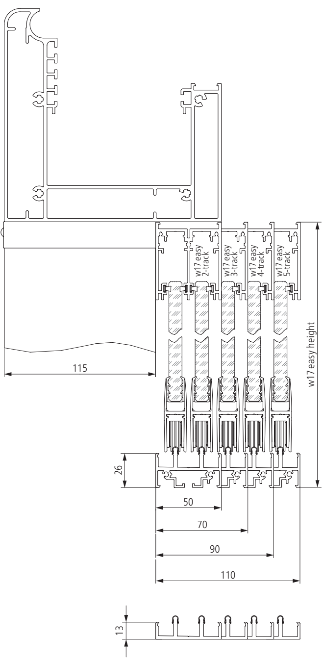
At the front behind posts, 2 to 5-track
