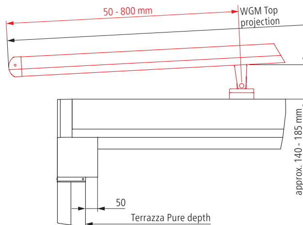
WGM Top with overhang
