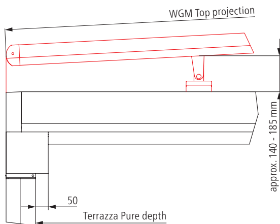
Standard without overhang
