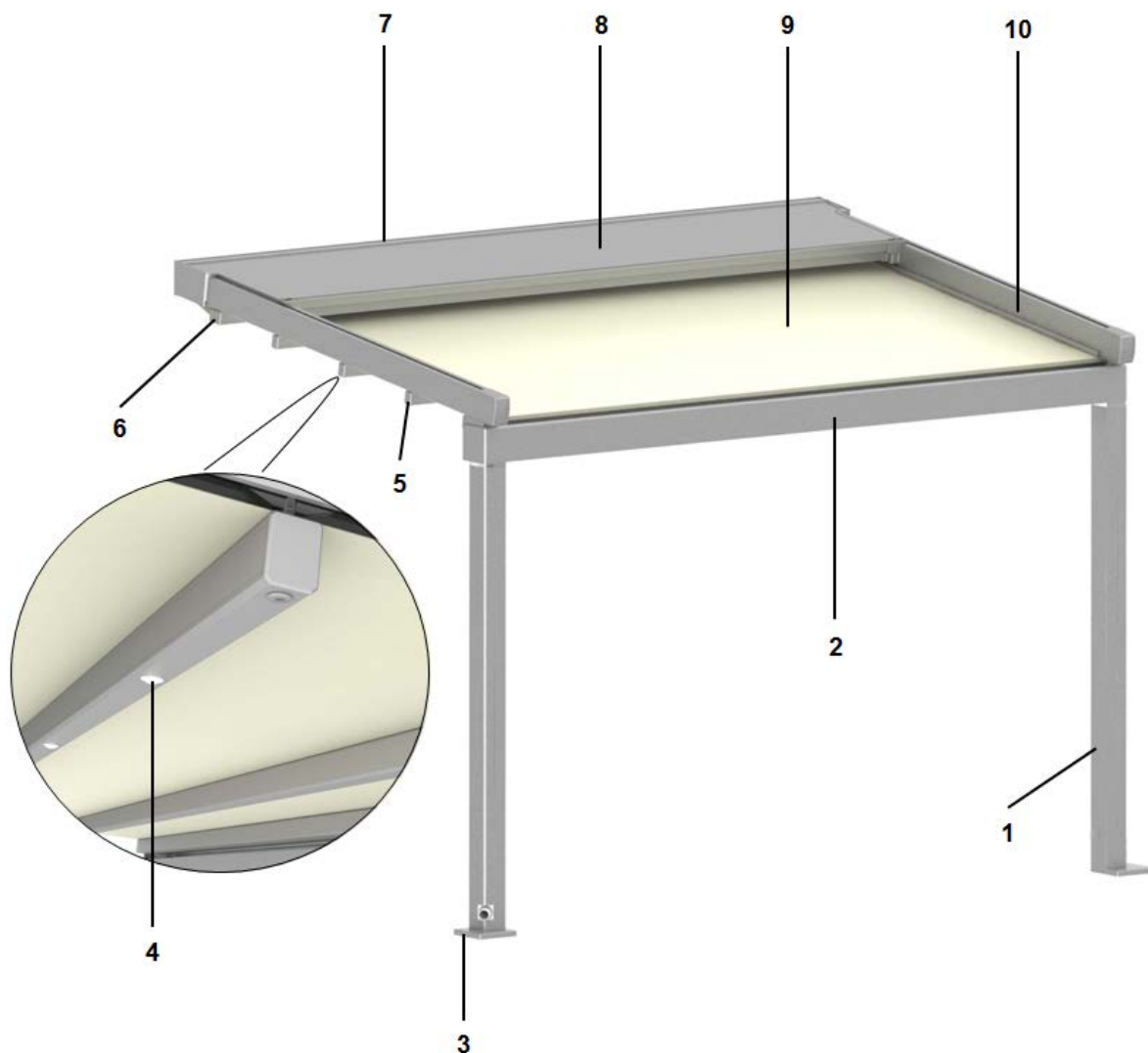
Figure 2: Schematic diagram of the PergoTex II Basic/ LED
