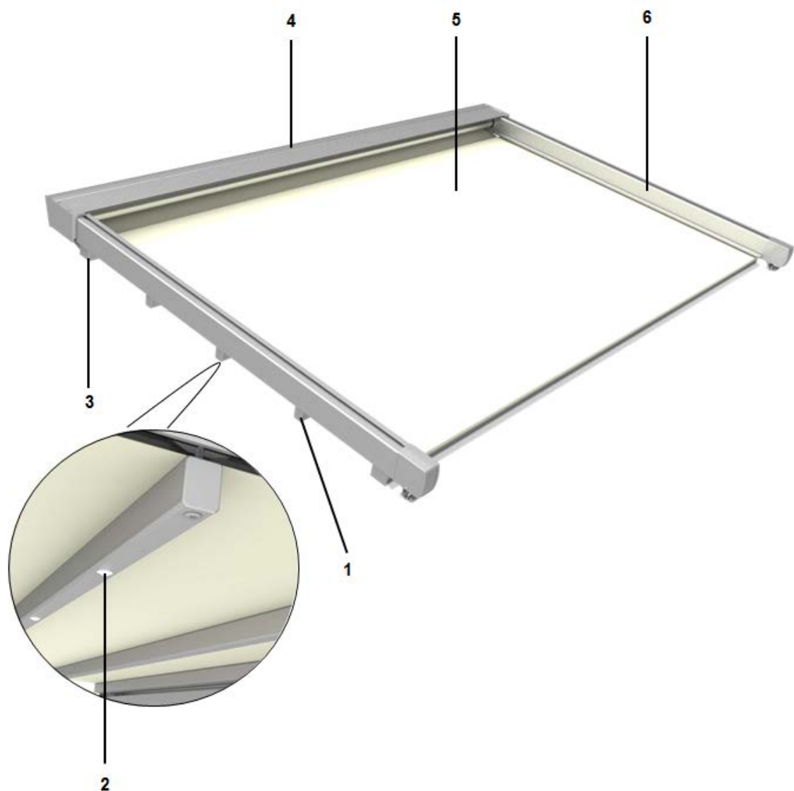
Figure 1: Schematic diagram of the PergoTex II Basic/ LED
